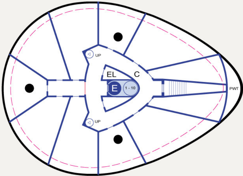
DECK 3: AIR, FOOD, WATER, FUEL
